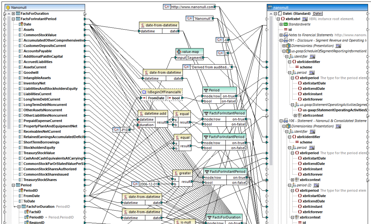
Mapping DB_to_XBRL.mfd
