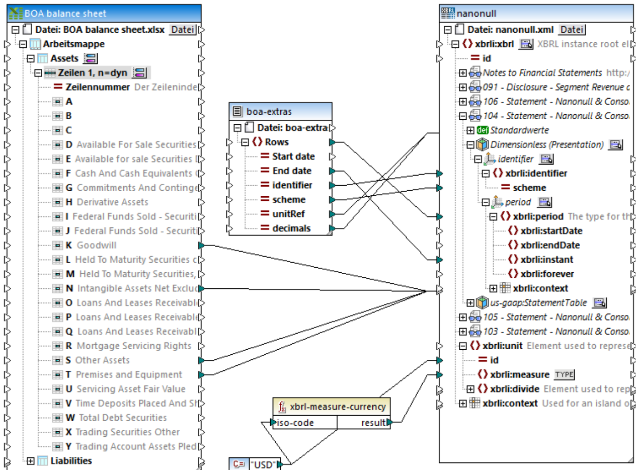
boa-balance-sheet.mfd Mapping
