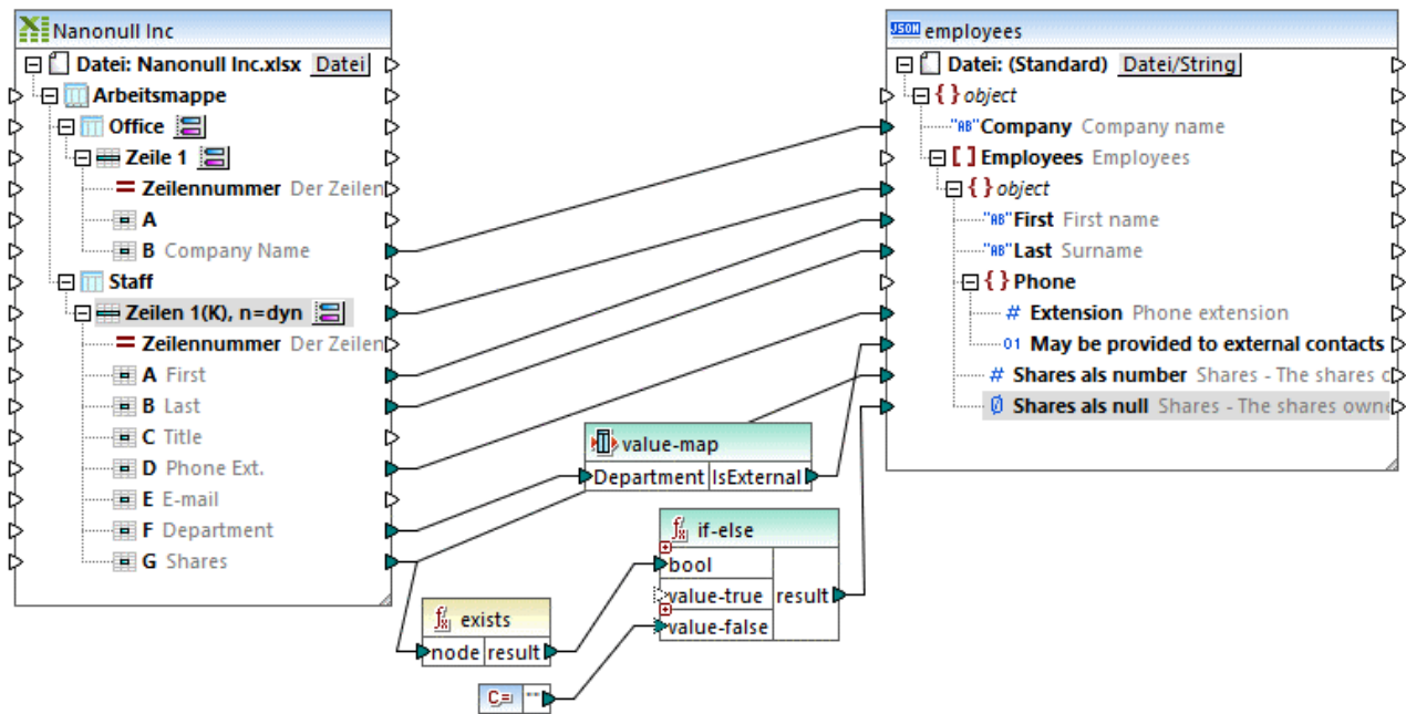
Excel_Company_To_JSON.mfd
